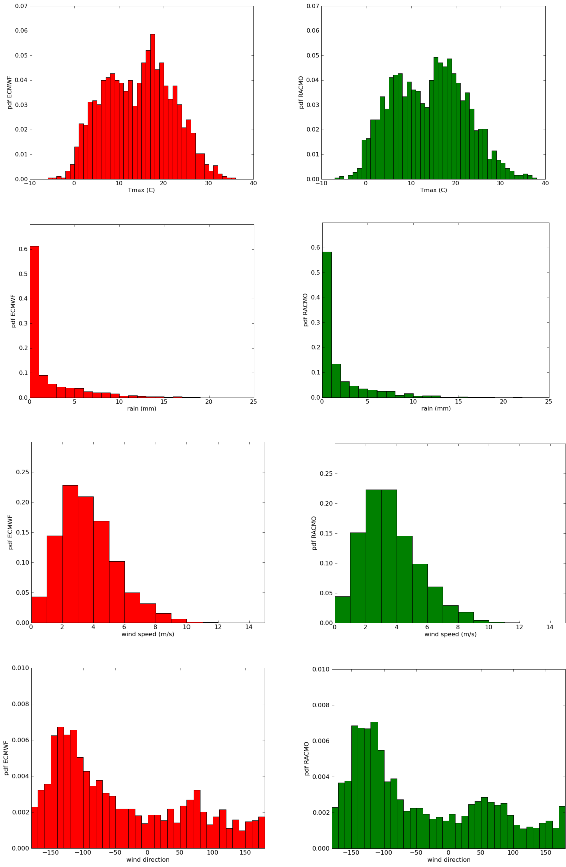
Figure 4. Probability density plots for 2003-2007, ECMWF and RACMO meteorology at Vredepeel.
