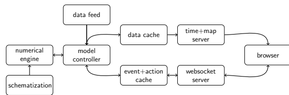
Figure 2. Architecture overview
