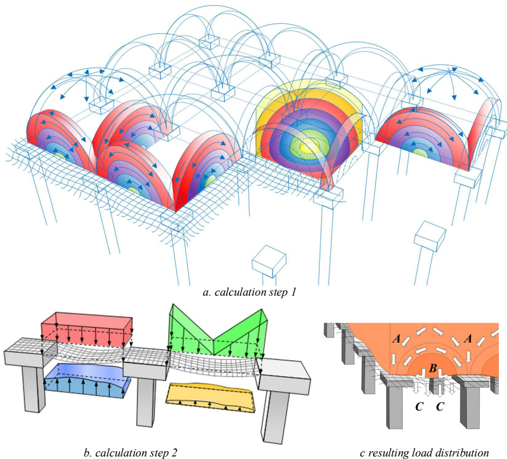
Figure 2: The new Concentric Arches model (Van Eekelen, 2015 and Van Eekelen et al., 2012b, 2013, 2015) consists of two steps: (a) step 1 calculates the load distribution in A and B+C and (b) step 2 calculates the GR strain that occurs in the GR strip between adjacent pile caps (c) resulting load distribution ( A , B , C ).
