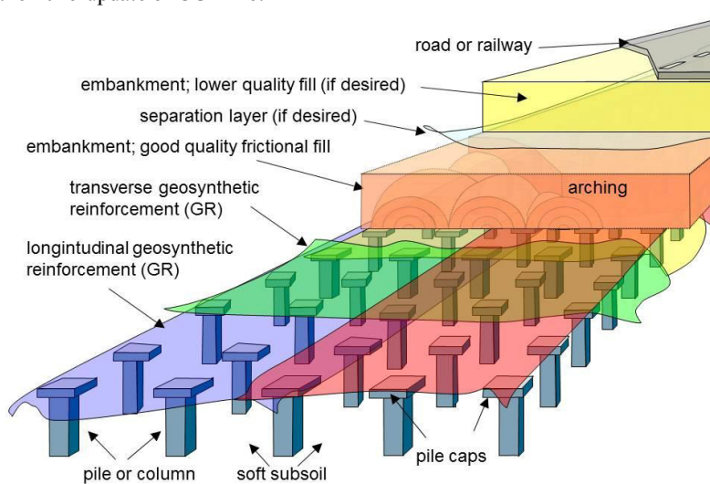
Figure 1: A basal reinforced piled embankment.
