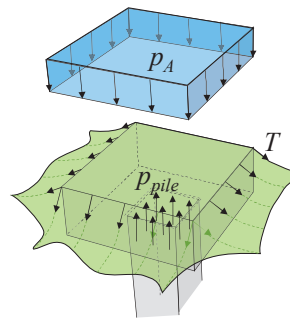
Figure 5: Loads on a pile cap: arching p_A (kPa), the tensile force T (kN/m) and the axial pile force p_{pile} , uniformly distributed (kPa).
