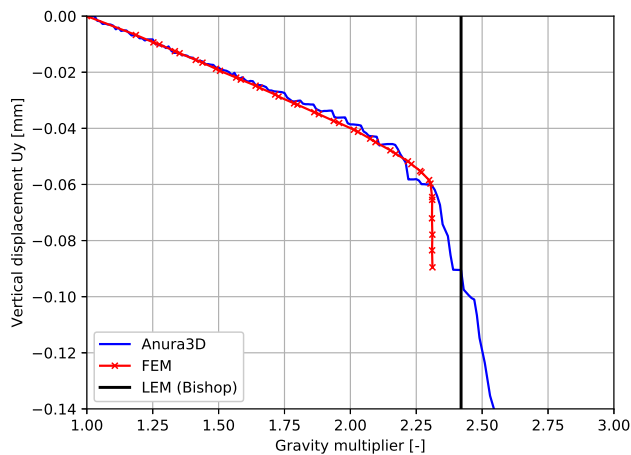
Figure 2: Comparison between FEM (Hicks & Wong 1988) MPM and LEM results for the vertical displacement of the slope crest.
