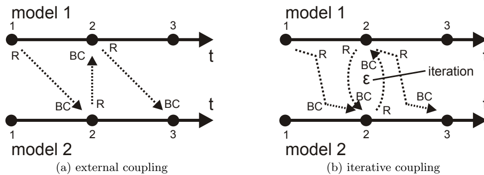
Figure 1: Functional principle of external coupling and iterative coupling of two models (after Becker, 2010). Abbreviations: R: result, BC: boundary condition, t: time, \varepsilon : convergence criterion.
