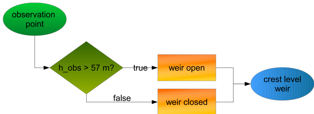
Figure 6: Flow chart for the control of the weir as modelled with RTC-Tools
