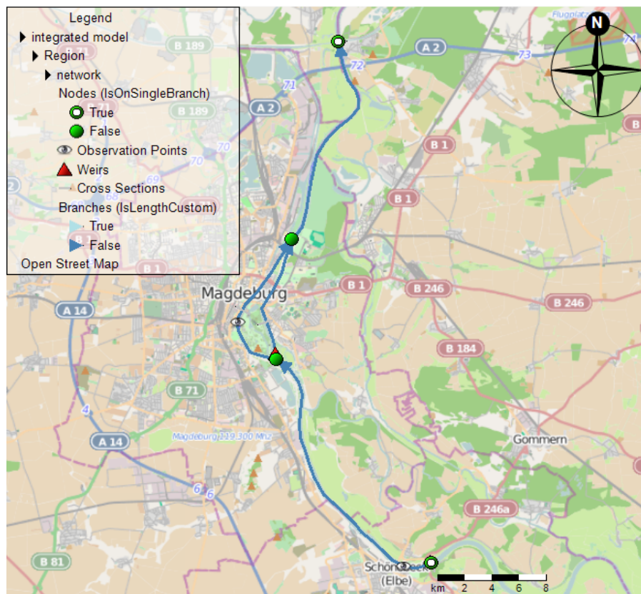
Figure 5: SOBEK open channel flow model network. Water flows from south to north. (Background map from www.openstreetmap.org .)
