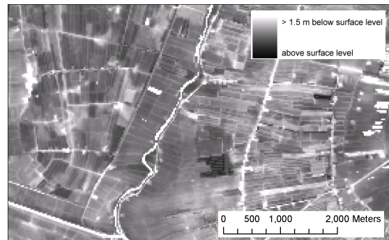
Figure 4. MIPWA model result: mean highest groundwater level.
