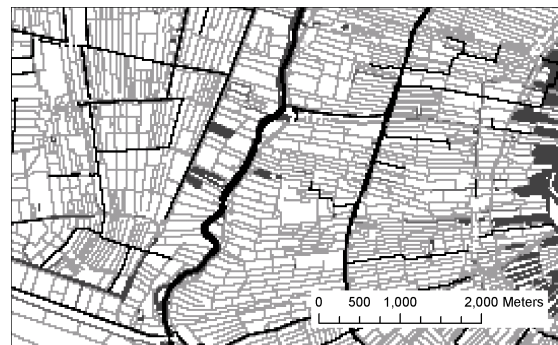
Figure 3. Representation of individual surface water bodies in the model. Scale ranges from light grey to black, from small ditch to river.
