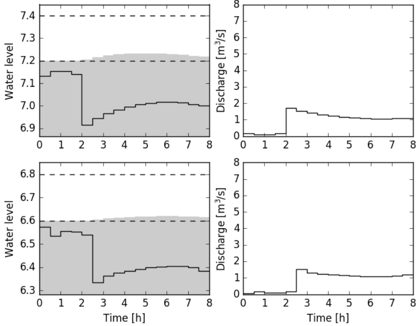
Figure 5 Water levels (grey) with weir height (black) and discharge in branches 5 and 6
