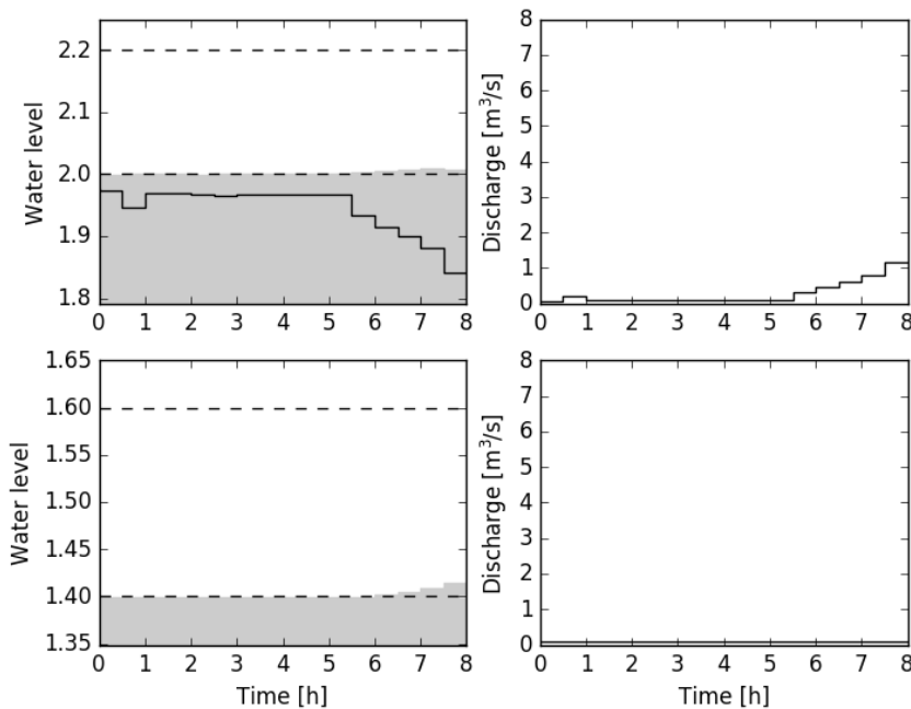
Figure 8 Water levels (grey) with weir height (black) and discharge in branches 11 and 12
