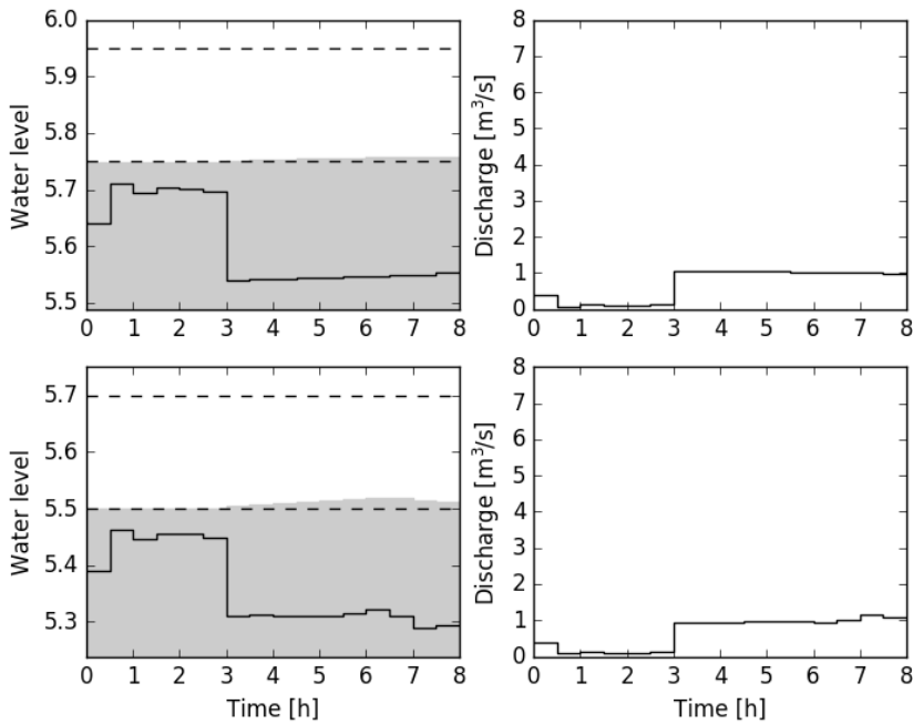
Water level and discharge in branch 7 and 8
