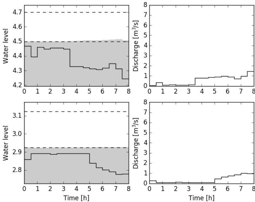
Figure 7 Water levels (grey) with weir height (black) and discharge in branches 9 and 10
