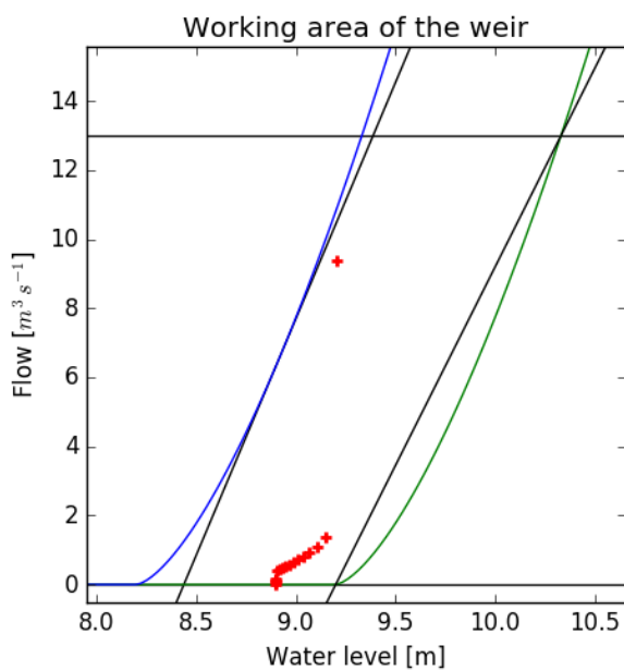
Figure 1 Working area of the weir: with blue and green line the non-linear flow head relations and with black line the actual constraints. The
