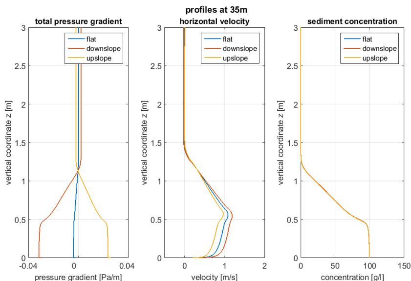
Figure C.18 Pressure gradient, velocity and concentration profile for x = 35m . Three cases: flat bed, downsloping bed and upsloping bed.
