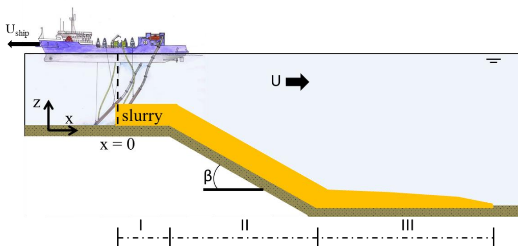
Figure 2.3 Situation sketch for hypothetical WID case, where slurry is mobilized and flows down a slope. It deposits when the bed becomes flat.
