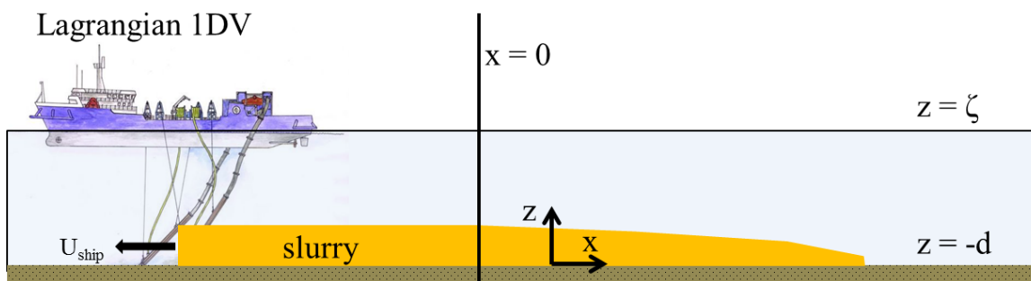
Figure 2.1 Sketch of Lagrangian 1DV domain for WID slurry computations. The initial conditions for the 1DV computation are applied at x=0 .
