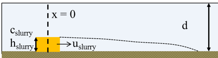
Figure 2.4 Initial slurry conditions at x=0 . The dashed line indicates a possible path for the slurry.
