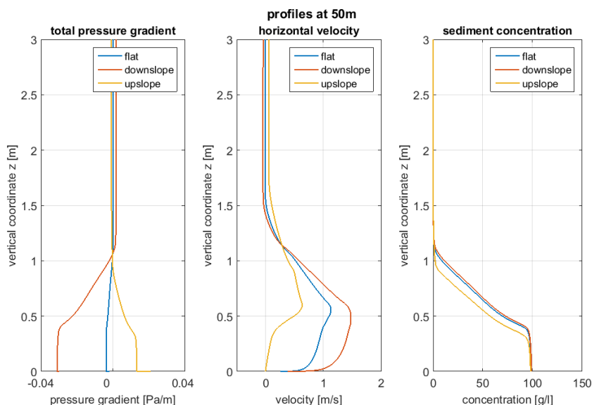
Figure C.19 Pressure gradient, velocity and concentration profile for x = 50m . Three cases: flat bed, downsloping bed and upsloping bed.
