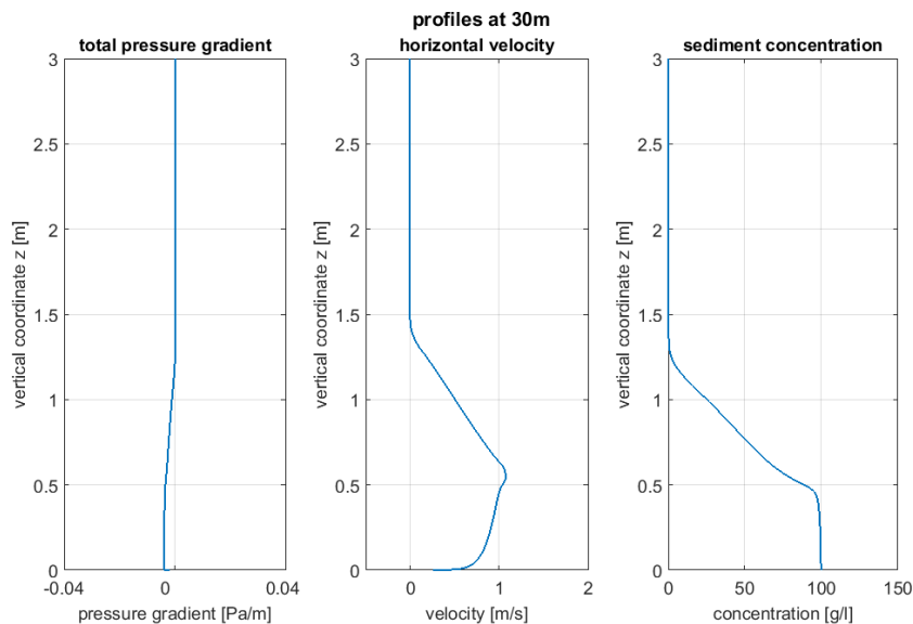
Figure C.17 Pressure gradient, velocity and concentration profile for x = 30m .
