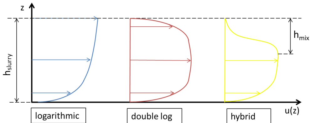
Figure 2.11 Available velocity profile shapes as initial condition for the 1DV model.
