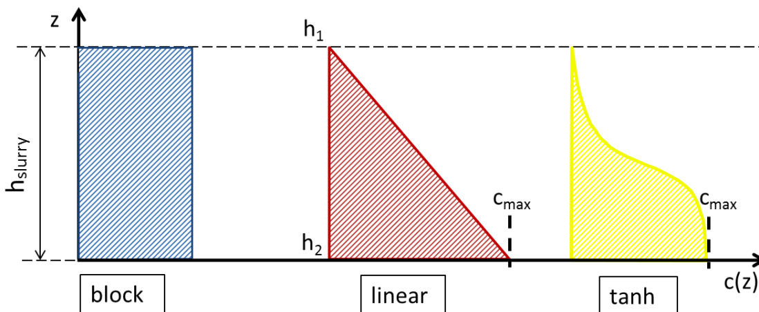
Figure 2.12 Available concentration profile shapes as initial condition for the 1DV model.
