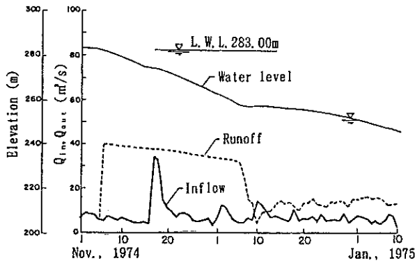
Fig.15 Calculated water level during the gate operation
