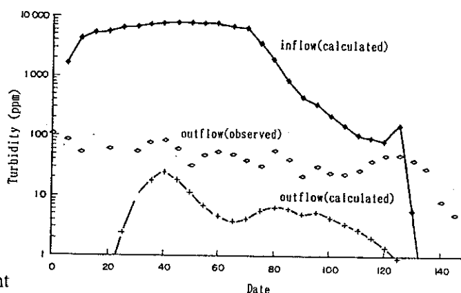
Fig.20 Comparison between calculated and observed fine sediment concentration during lower water level
