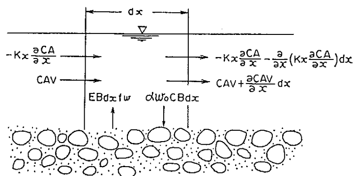
Fig.14 Schematics of mass conservation of fine sediment
