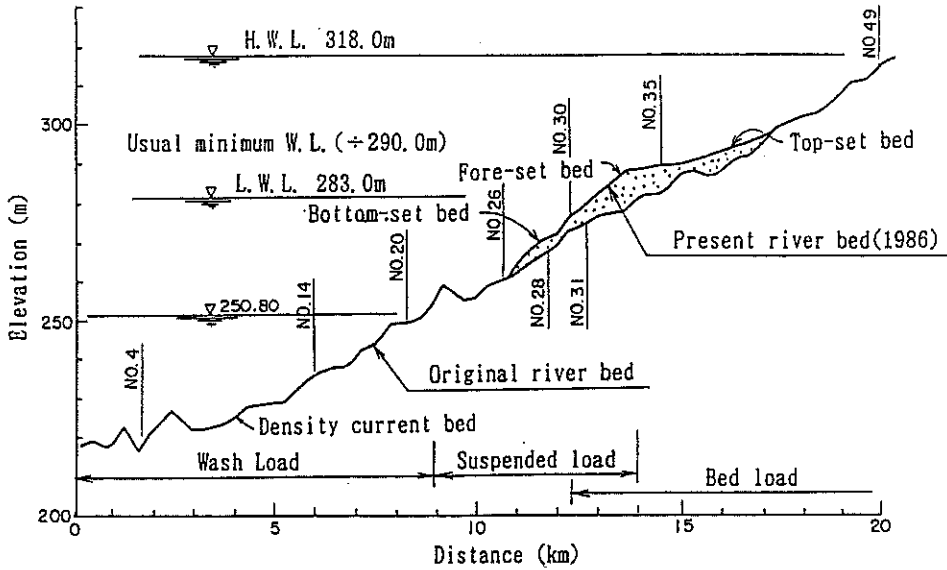
Fig.1 Longitudinal bed profile of Ikehara reservoir
