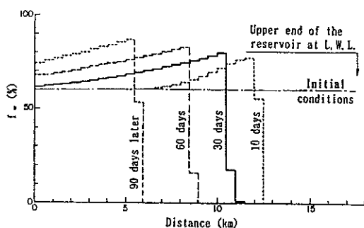
Fig.19 Turbid material content of sediment at the surface layer of reservoir bed
