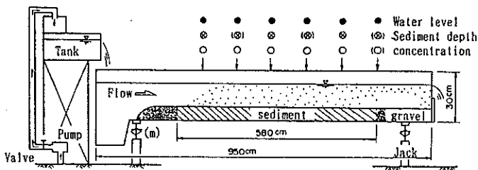
Fig.7 Laboratory experiment set-up
