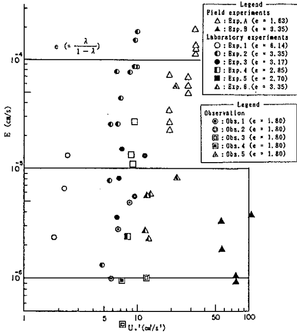
Fig.9 Relation between shear velocity and erosion velocity
