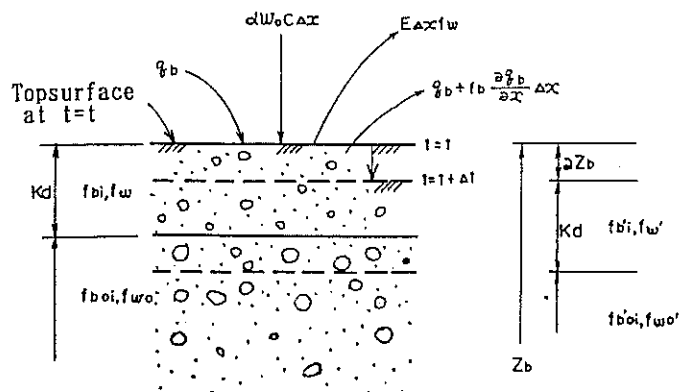
Fig.13 Definition sketch
