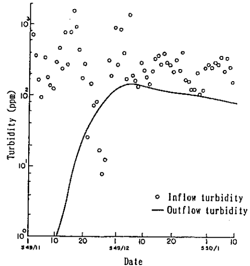
Fig.16 Calculated results of turbidity at the inflow section and outflowing water of Ikehara reservoir
