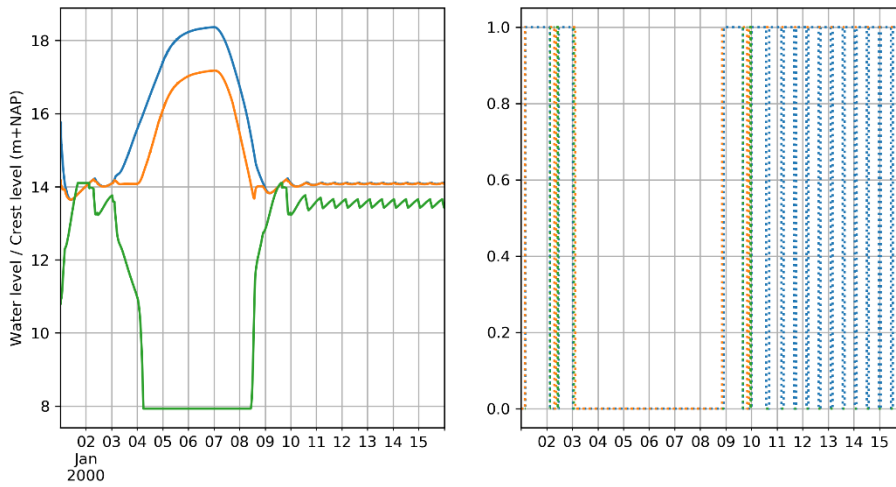
— [Input]LA_1.30_L_LMW-H_Heel-beneden/water_level — [Input]MA_100.75_R_LMW-H_Belfeld-boven/water_level — [Output]ST_Belfeld/CrestLevel -.- [Status]stuw_Belfeld/Conditie_Heel_1 -.- [Status]stuw_Belfeld/Conditie_Heel_2 -.- [Status]stuw_Belfeld/Conditie_Belfeld
