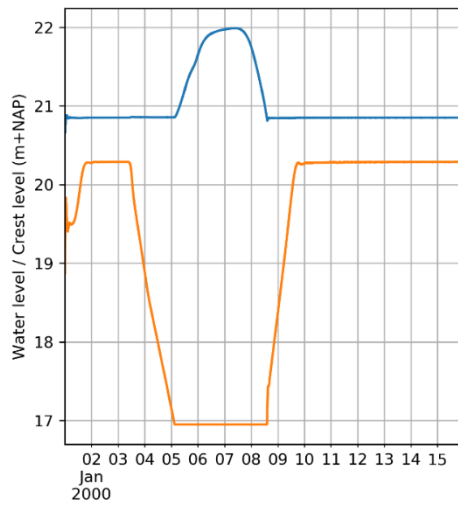
— [Input]MA_67.30_L_LMW-H_Heel-boven/water_level — [Output]ST_Linne/CrestLevel
