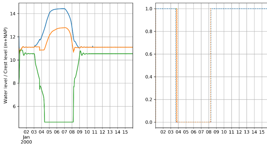
— [Input]MA_132.10_R_LMW-H_Well-dorp/water_level — [Input]MA_144.96_R_LMW-H_Sambeek-boven/water_level — [Output]ST_Sambeek/CrestLevel -.- [Status]stuw_Sambeek/Conditie_Well_1 -.- [Status]stuw_Sambeek/Conditie_Well_2 -.- [Status]stuw_Sambeek/Conditie_SambeekBoven_1 -.- [Status]stuw_Sambeek/Conditie_SambeekBoven_2
