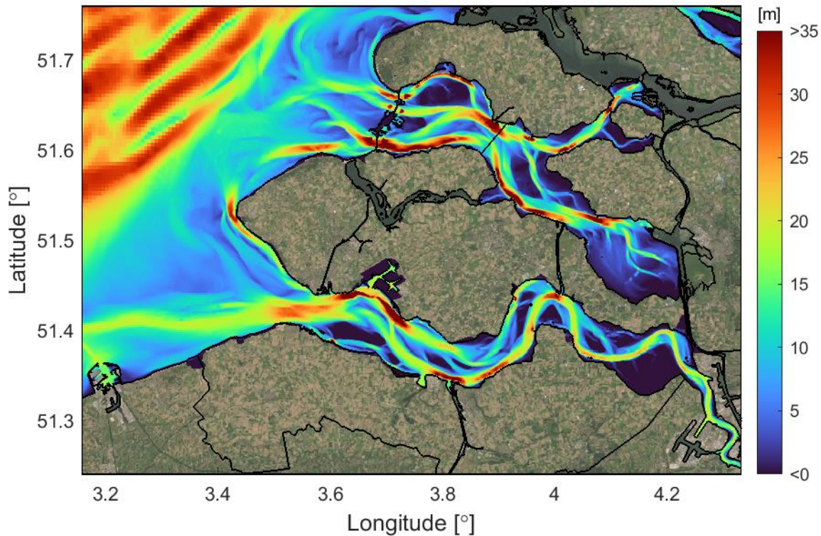
Figure 2.12 DCSM-FM model bathymetry in the South-western Delta (depths relative to MSL).
