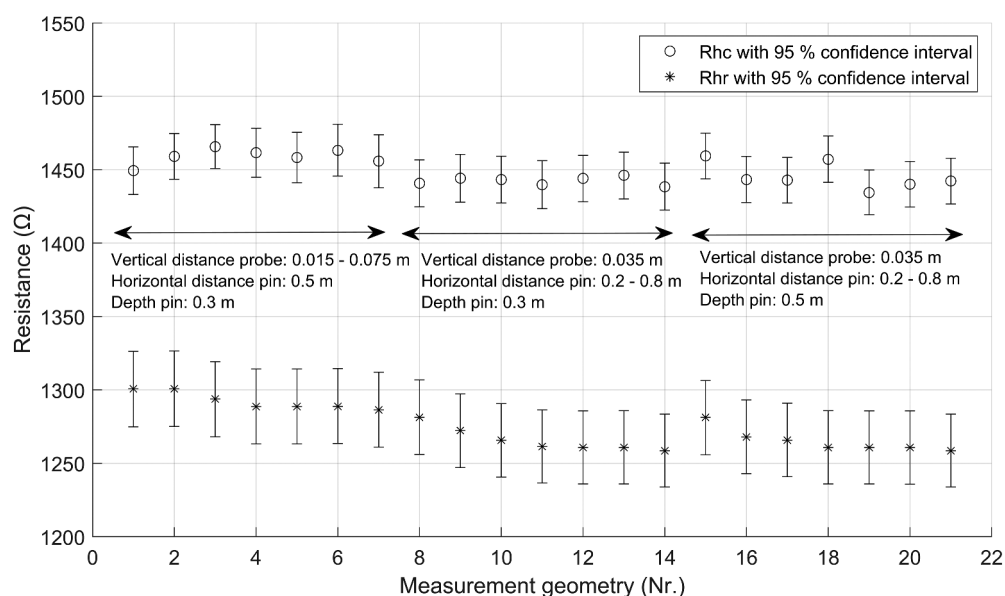
Figure 11. The calibrated electrical resistance of the leakage ( R_{hc} ) and the reference electrical resistance of the leakage ( R_{hr} ) at the measurement geometries.
