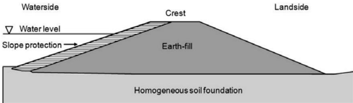
(a) Homogene dijk
