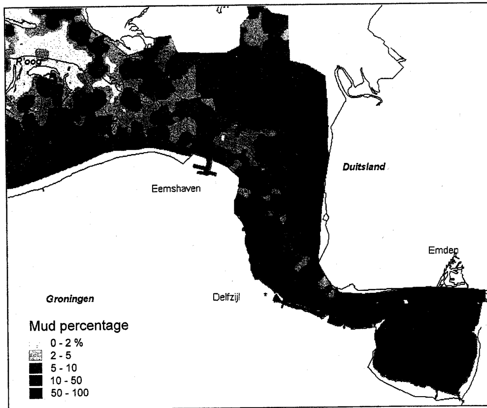
Fig. 1. SEDIMAP output showing the mud percentages of samples from the Eems/Dollard Estuary, Dutch Waddenzee.
