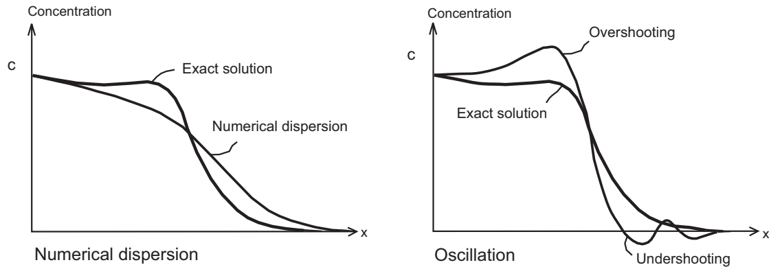
Figure 1: Schematisation of numerical dispersion and oscillation.
