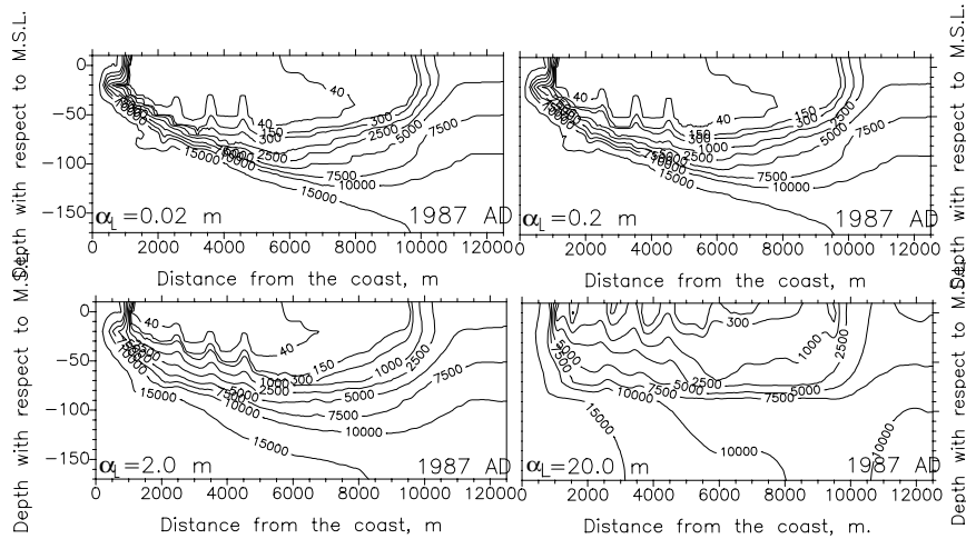
Figure 2: Chloride distributions (in mg\ Cl^-/l ) in 1987 in a cross-section of the sand-dune area of Amsterdam Waterworks, the Netherlands, calculated with MOC [Konikow & Bredehoeft, 1978] (adapted for density differences to model vertical cross-sections [Oude Essink, 1996]) for four different longitudinal dispersivities: \alpha_L=0.02\ m , \alpha_L=0.2\ m , \alpha_L=2.0\ m and \alpha_L=20.0\ m . A thick freshwater lens is only simulated for small dispersivities.
