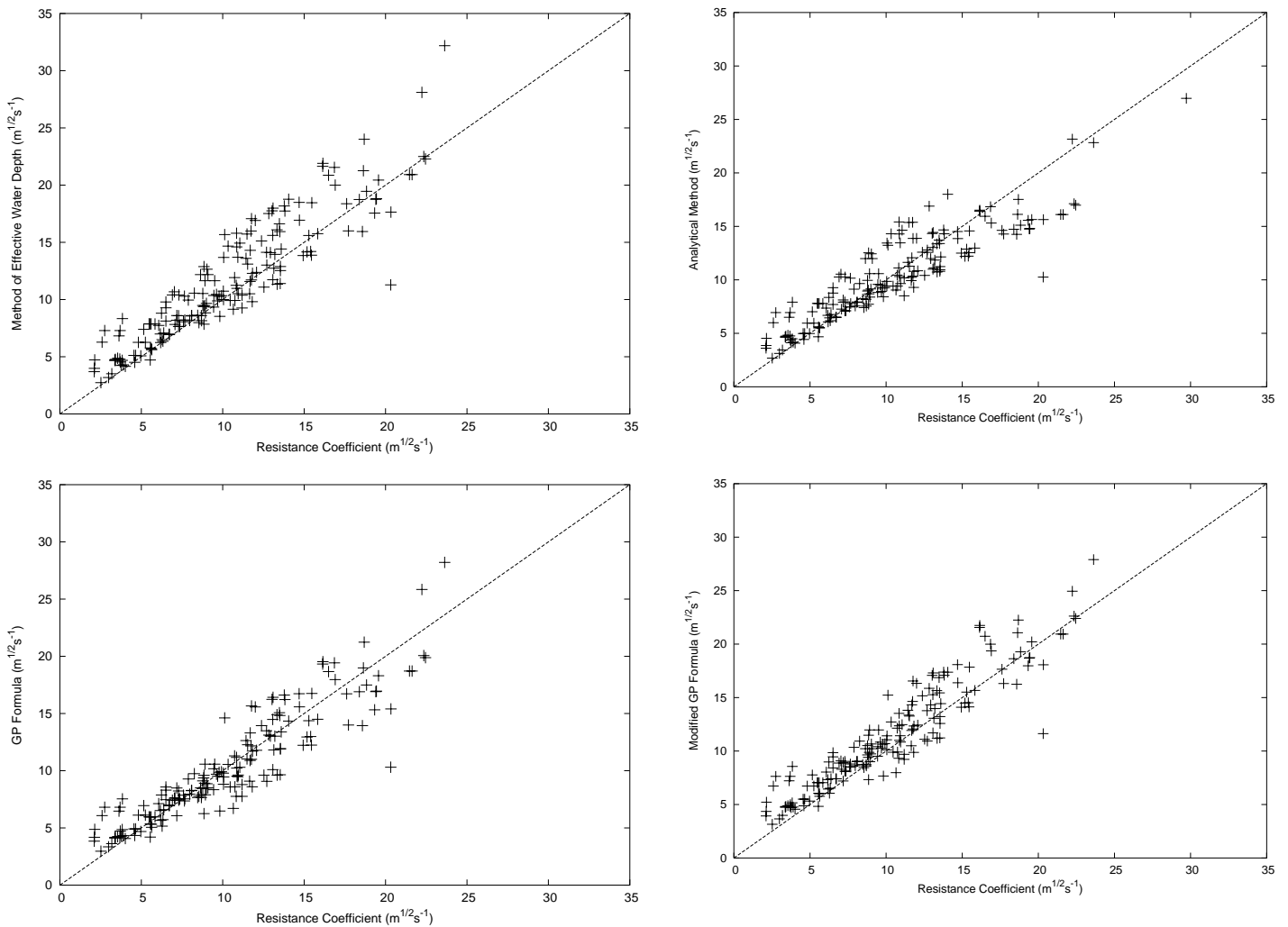
Figure 6 Scatter plots for the four equations for experimental flume data. (a) upper left: method of effective water depth, Eq. (19), (b) upper right: analytical solution method, Eq. (44), (c) lower left: original GP-formula, Eq. (71) and (d) lower right: modified GP-formula, Eq. (74).
