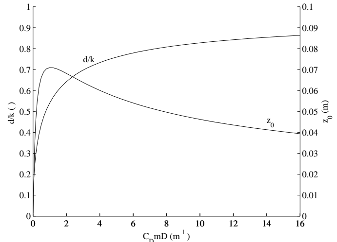
Figure 4 The dimensionless zero-plane displacement, d/k (left axis), and the roughness height for the top of the vegetation, z_0 (right axis), as function of C_D m D . h = 2 \text{ m} , k = 0.5 \text{ m} , C_D = 1 .
