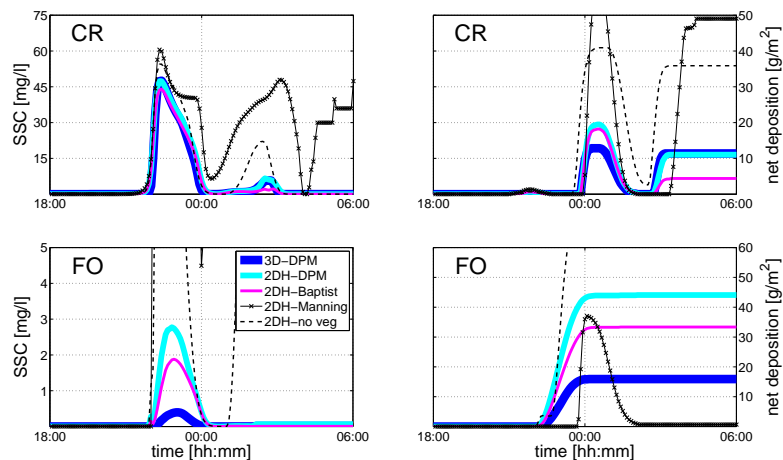
Figure 6. Simulated suspended sediment concentrations and cumulative deposition rates for points located within the creek (CR) and in the forest (FO). Results are from the same models as in Figure 4.
