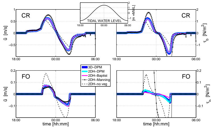
Figure 4. Simulated depth-averaged flow velocities and bed shear stresses for points located within the creek (CR) and in the forest (FO). Results show the effect of different vegetation representations (DPM, Baptist, Manning) and different model settings (3D with depth-variable vegetation or 2DH with depth-uniform vegetation). For reference, the results of a run without vegetation are included (no veg).
