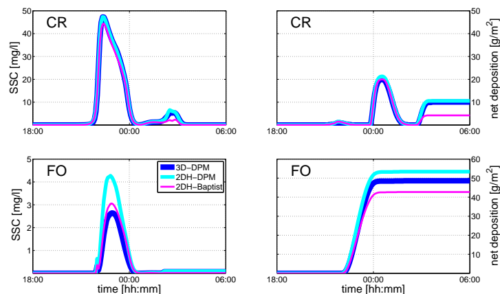
Figure 7. Adjusted model predictions after calibration of each model in the sediment settling velocity.
