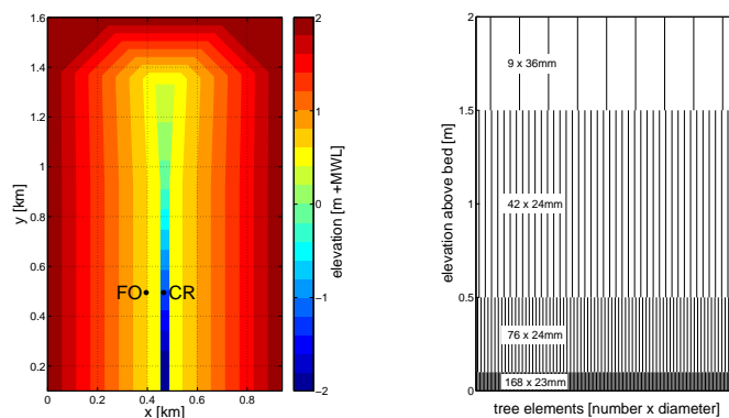
Figure 3. Bathymetry of the schematized study area with monitoring locations in the FOrest and CReek (left) and the measured geometry of the root system of a single Rhizophora tree (right).
