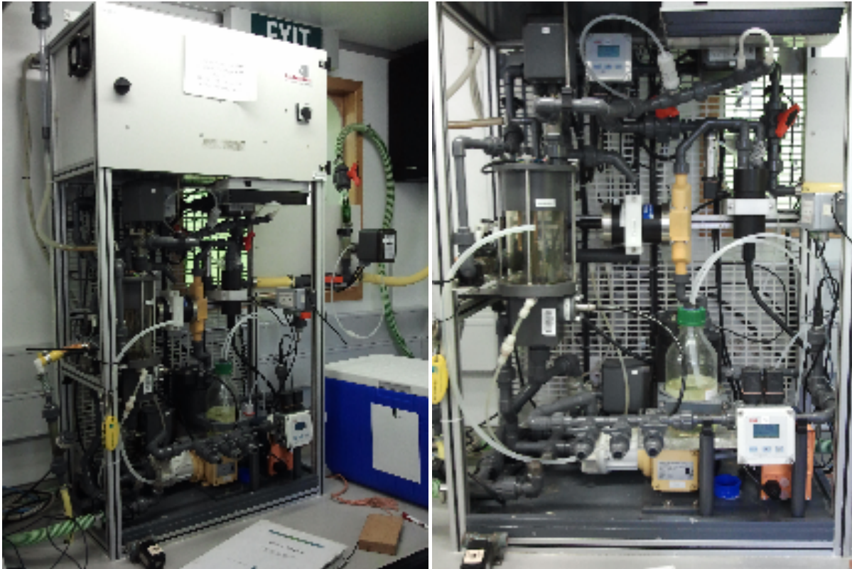
FerryBox installation at Zirfaea during World Hydrography Day 2013 ship visit in Scheveningen
