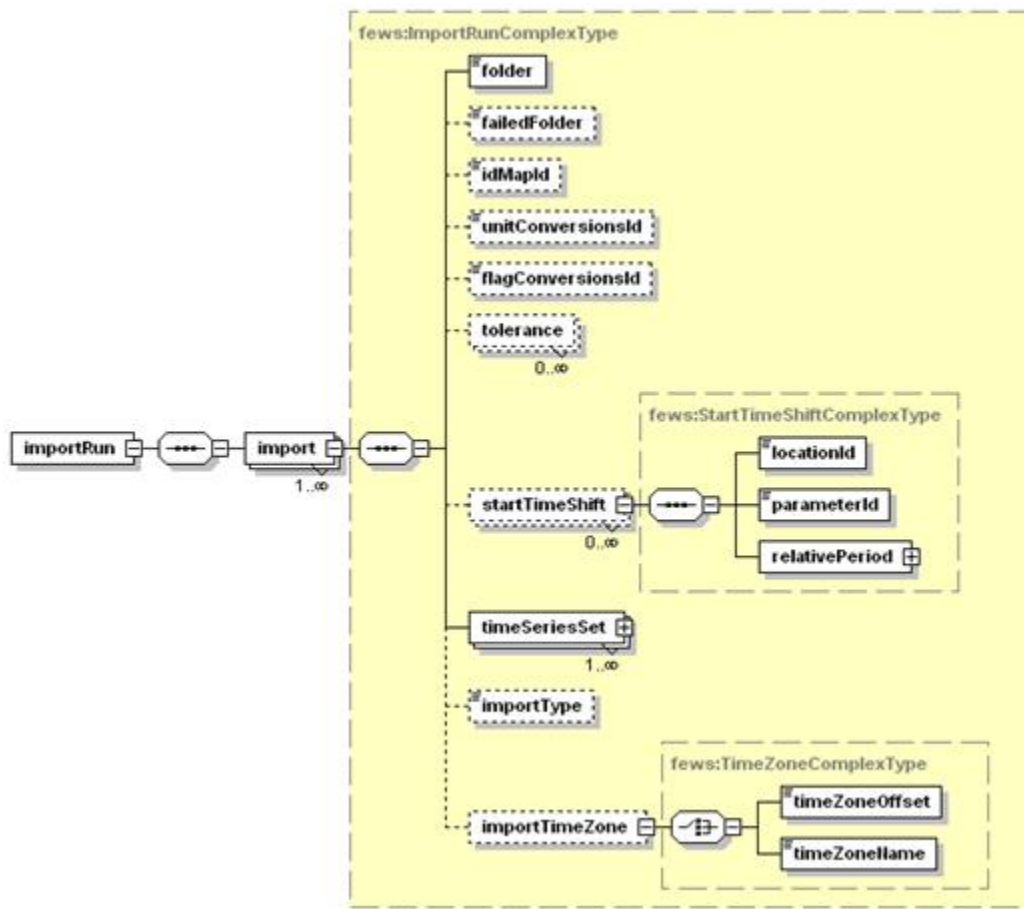
Figure 63 Elements of the EAIImport configuration.
