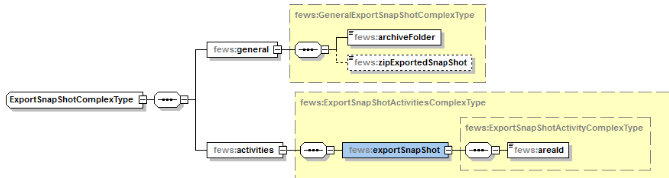
Figure 4.9 Delft-FEWS export configuration for archiving database snap shots
